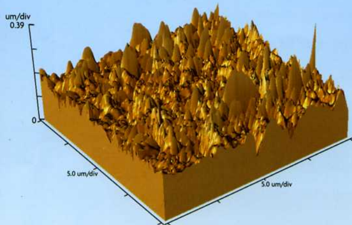
Microscope Image Unprotected glass after exposure to typical shower conditions
