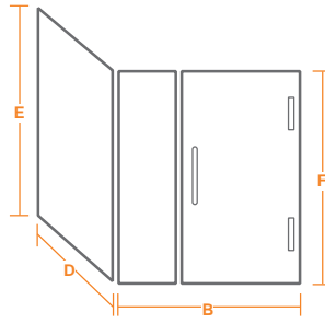
7. Door w/Inline Panel 90° Full Panel Return
