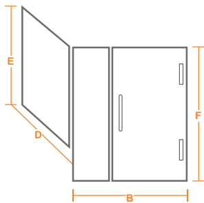
6. Door w/Inline Panel 90° Half Panel Return
