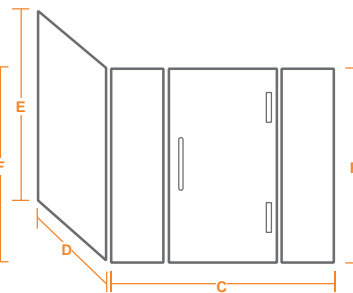
11. Door w/2 Inline Panels, 90° Full Panel Return
