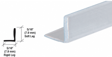
Translucent Vinyl "L" Seal
